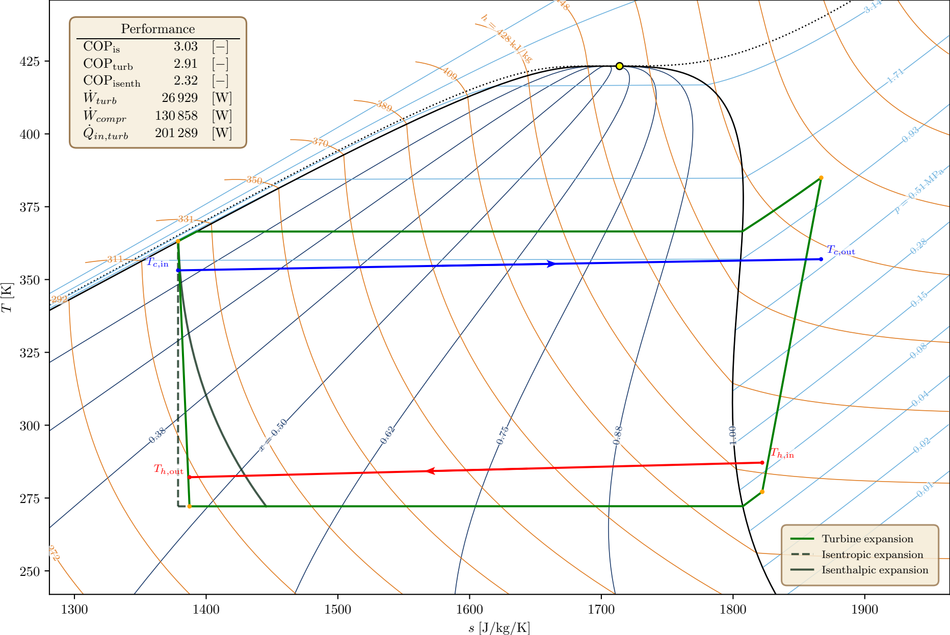
Conceptual Heat Pump Cycle – R1234ze(Z)
